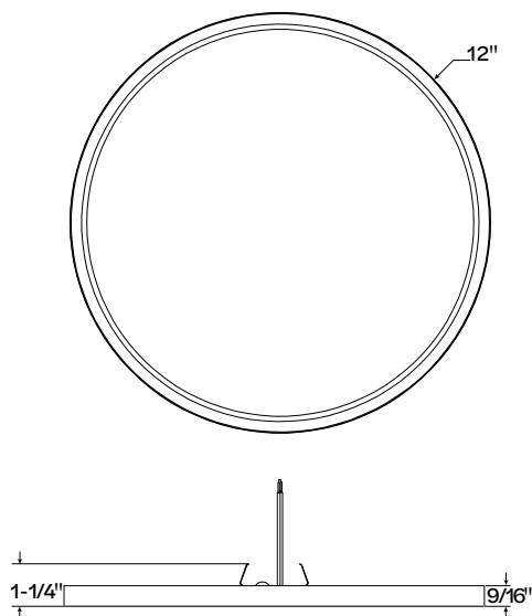
12" Surface Mount Disk Light- DSK-12-CS-120V
