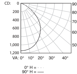
99621, CDL8FR30/950/RTJB/LED
